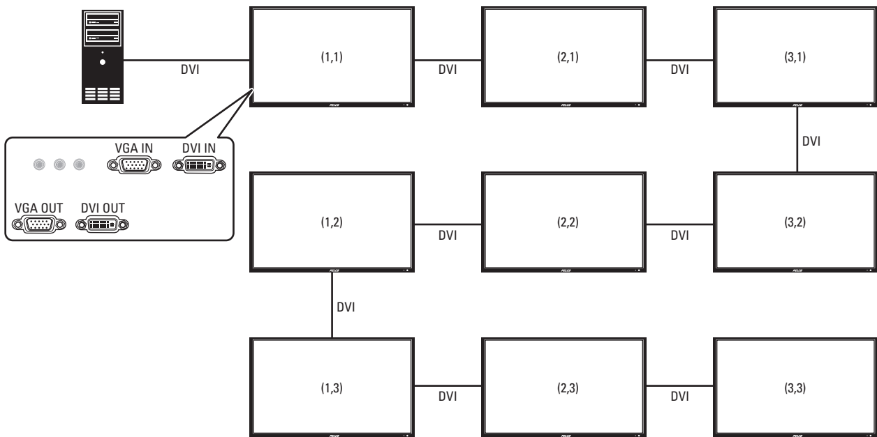
Figure 9. DVI Connection
